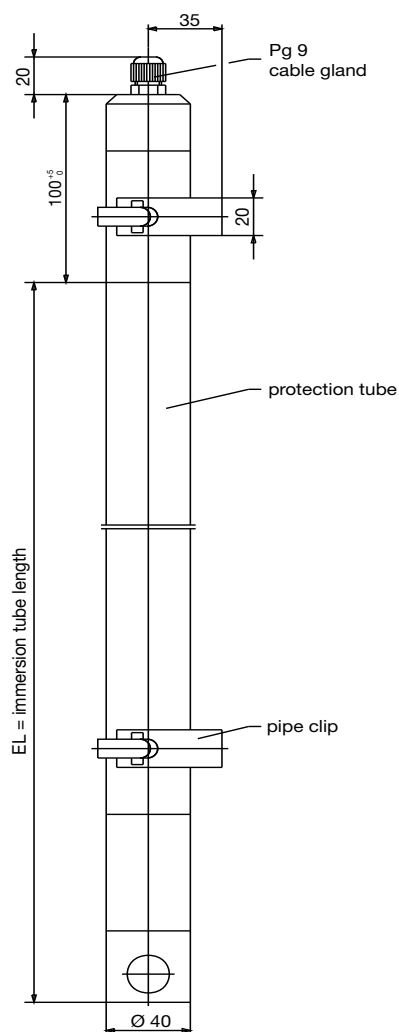
Immersion fitting 202820/40-...
