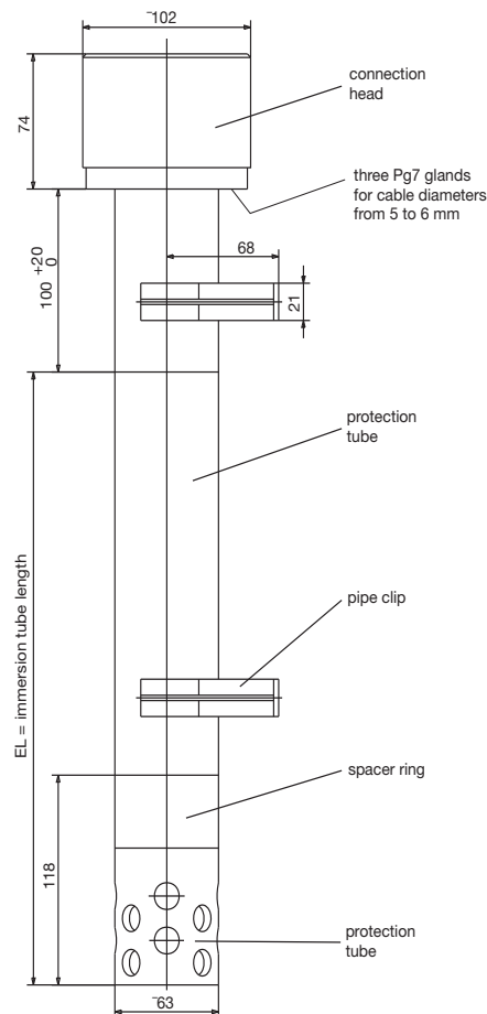
Immersion fitting 202820/63-...
