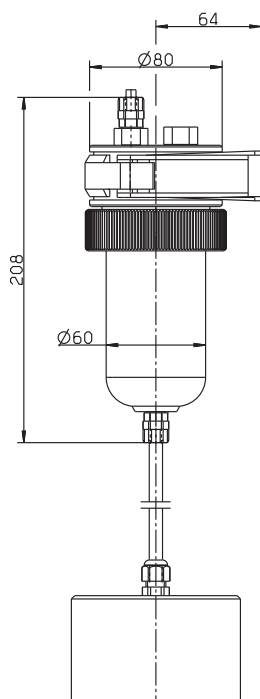
KCl reservoir, pressure-tight, suitable for wall mounting Sales No. 20/00060254; to set up an electrolyte bridge or when using KCl-filled electrodes
