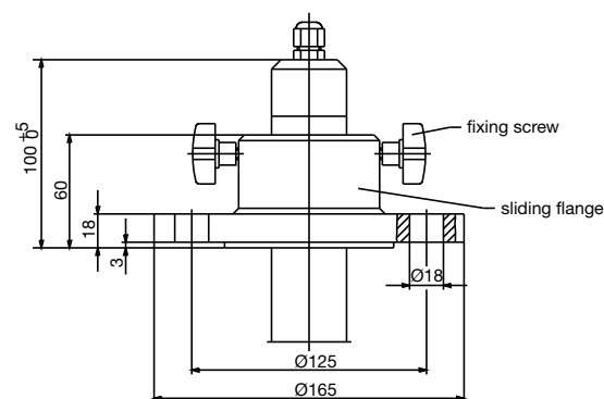
Flange DN50, Sales No. 20/00083376
