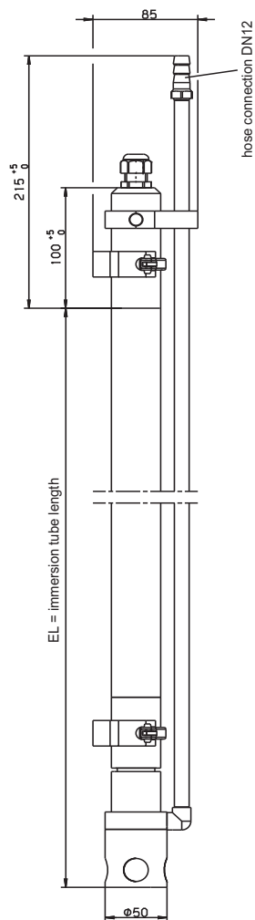
Cleaning nozzle, code 078
