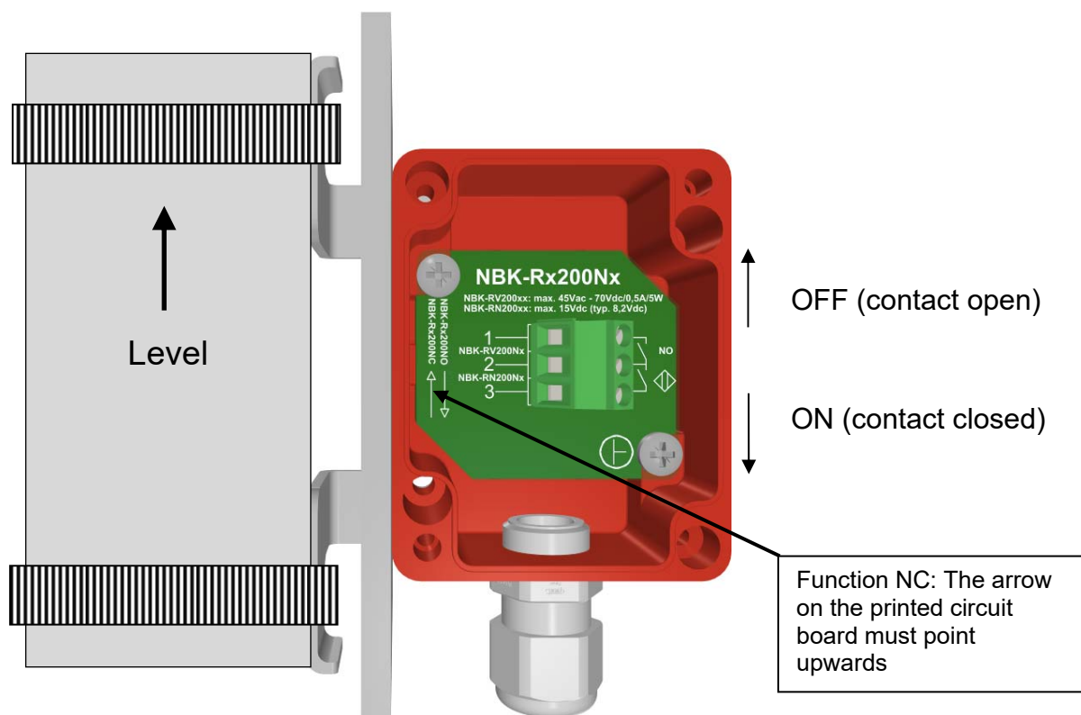
Mounting NBK-RN200NC and NBK-RV200NC
