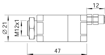
Right Angle Mirror for Air Cooling Jacket and Air Purge Jacket only (XXXMIACRAJ)
