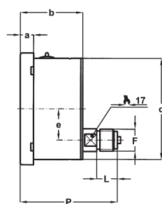
BACK CONNECTION MOUNTING
