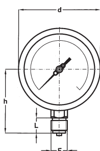
LOWER CONNECTION MOUNTING
