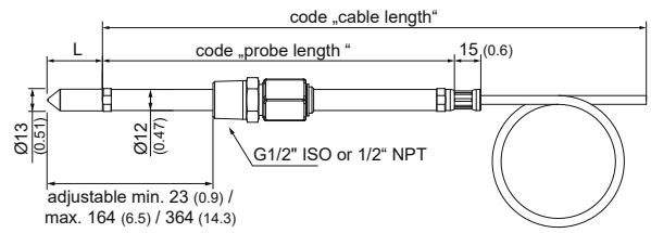
Type: T10 Remote probe 20 bar (300 psi) with sliding fitting for assembly / disassembly under pressure
