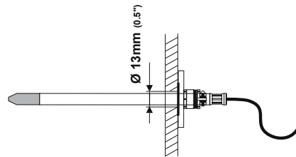
Horizontal mounting
