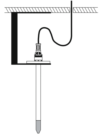
Vertical mounting
