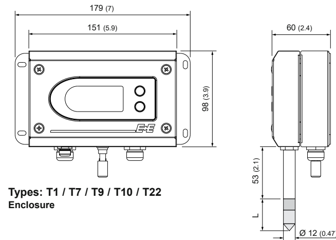
Type: T1 Wall mount
